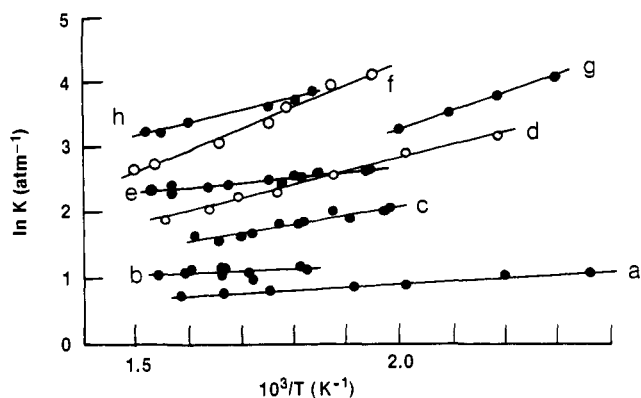
Figure 2. van't Hoff plots for proton-transfer equilibria between the reactants: a. \text{C}_6\text{H}_5\text{NH}_2\text{H}^+ + 2\text{-Fpyridine} ; b. \text{CH}_3\text{OH}_2^+ + \text{C}_6\text{H}_6 ; c. i\text{-C}_3\text{H}_7^+ + \text{CH}_3\text{OH} ; d. \text{C}_6\text{H}_7^+ + \text{CH}_3\text{CHO} ; e. \text{CH}_3\text{CNH}^+ + \text{C}_6\text{H}_5\text{CH}_3 ; f. \text{C}_6\text{H}_7^+ + \text{CH}_3\text{CN} ; g. \text{C}_6\text{H}_7^+ + \text{CH}_3\text{SH} ; h. \text{CH}_3\text{CNH}^+ + \text{C}_2\text{H}_5\text{CN} .
