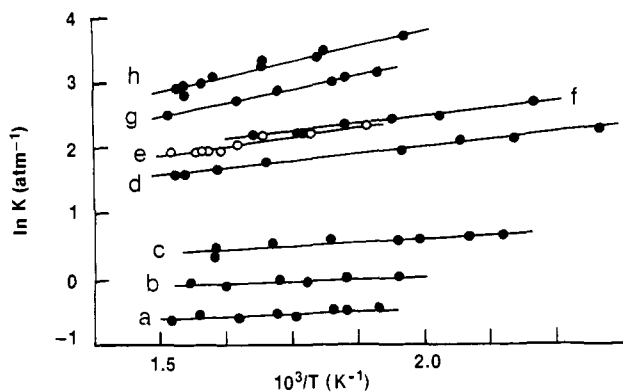
Figure 7. van't Hoff plots for proton-transfer equilibria between the reactants: a. i -C 4 H 9 + + i -C 3 H 7 CN; b. (CH 3 ) 2 OH + + C 2 H 5 CN (intercept arbitrary); c. CF 3 CH 2 NH 3 + + NH 3 ; d. oxazoleH + + 2-Fpyridine; e. CH 3 CHOH + + CH 3 CN; f. CF 3 CH 2 NH 3 + + c -C 3 H 5 COCH 3 ; g. (CH 3 ) 2 OH + + i -C 3 H 7 CN (intercept arbitrary); and h. c -C 3 H 5 COCH 3 + + pyrrole.
