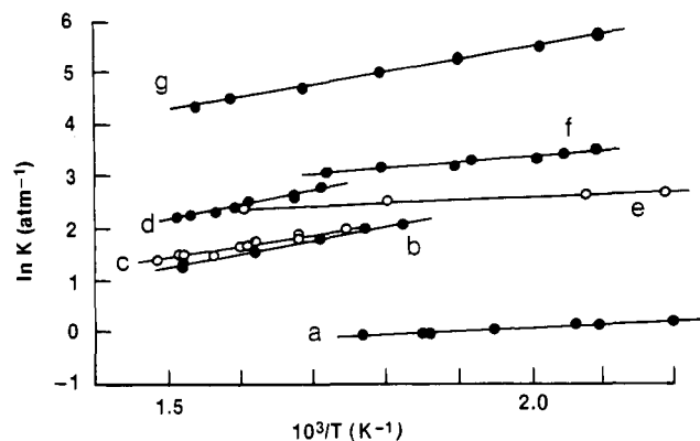
Figure 11. van't Hoff plots for proton-transfer equilibria between the reactants: a. pyridineH + + i -C 4 H 9 NH 2 ; b. (C 2 H 5 ) 2 COH + + NH 3 ; c. (CH 3 ) 2 SH + + CF 3 CH 2 NH 2 ; d. CH 3 COOC 2 H 5 H + + NH 3 ; e. CH 3 NH 3 + + 3-Fpyridine; f. t -C 3 H 7 NH 3 + + i -C 4 H 9 NH 2 ; and g. (CH 3 ) 2 NH 2 + + (CH 3 ) 3 N.
