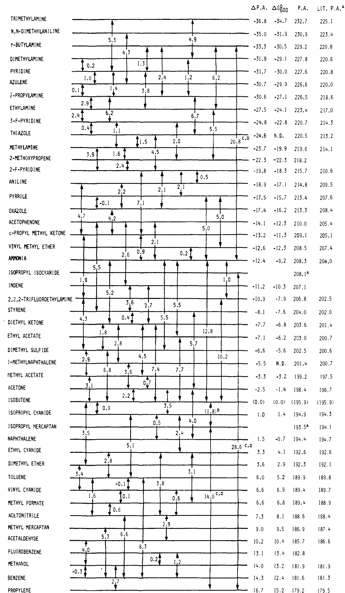
Figure 14. Interconnecting ladder of proton-transfer thermochemistry. Values in an arrow show \Delta H^{\circ} (kcal/mol), for AH^{+} + B \rightarrow BH^{+} + A , where A and B are the top and bottom compounds connected by the arrow: (a) from ref 1, (b) from ICR values, ref 1, (c) not included in the evaluated network and (d) from condensation equilibria.
