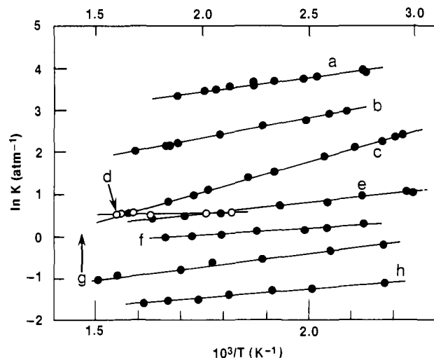
Figure 13. van't Hoff plots for proton-transfer equilibria between the reactants: a. 2-Fpyridine \text{H}^+ + 2-methoxypropene; b. \text{CH}_3\text{CHOC}_2\text{H}_5^+ + 2-Fpyridine; c. 2-methoxypropene \text{H}^+ + \text{C}_2\text{H}_5\text{NH}_2 ; d. \text{CH}_3\text{OH}_2^+ + \text{C}_6\text{H}_5\text{F} ; e. 2-methoxypropene \text{H}^+ + 3-Fpyridine; f. \text{CH}_3\text{CHOC}_2\text{H}_5^+ + oxazole; g. \text{C}_6\text{H}_7^+ + \text{C}_6\text{H}_5\text{F} (upper scale); and h. 2-methoxypropene \text{H}^+ + \text{CH}_3\text{NH}_2 .
