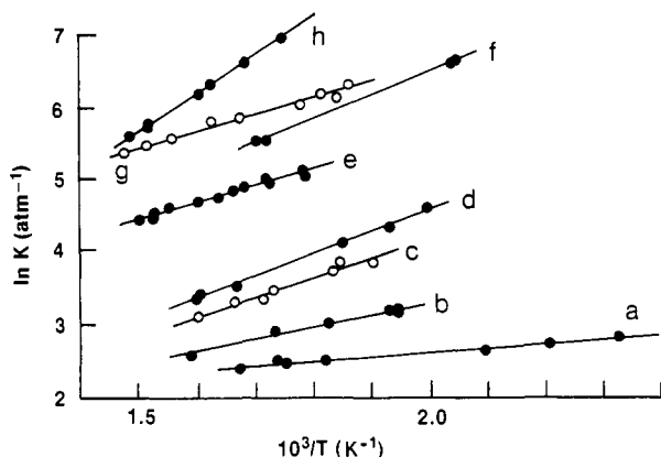
Figure 10. van't Hoff plots for proton-transfer equilibria between the reactants as follows: a. i -C 3 H 7 NH 3 + + pyridine; b. C 2 H 5 NH 3 + + t -C 3 H 7 NH 2 ; c. (CH 3 ) 2 SH + + NH 3 ; d. 3-FpyridineH + + t -C 3 H 7 NH 2 ; e. c -C 3 H 5 COCH 3 H + + C 6 H 5 NH 2 ; f. C 2 H 5 NH 3 + + i -C 4 H 9 NH 2 ; g. NH 4 + + pyrrole; and h. t -C 4 H 9 NH 3 + + CF 3 CH 2 NH 2 .
