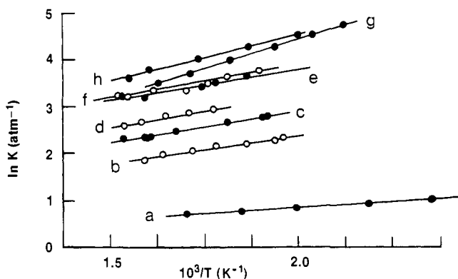
Figure 4. van't Hoff plots for proton-transfer equilibria between the reactants: a. \text{CH}_3\text{NH}_3^+ + \text{thiazole} ; b. \text{HCOOCH}_3\text{H}^+ + \text{C}_2\text{H}_5\text{CN} ; c. i\text{-C}_3\text{H}_7\text{CNH}^+ + (\text{CH}_3)_2\text{CO} ; d. \text{C}_2\text{H}_5\text{CNH}^+ + i\text{-C}_3\text{H}_7\text{CN} ; e. \text{CH}_2\text{CHCNH}^+ + \text{CH}_3\text{OCH}_3 ; f. (\text{CH}_3)_2\text{COH}^+ + 1\text{-methyl-naphthalene} ; g. \text{thiazoleH}^+ + i\text{-C}_3\text{H}_7\text{NH}_2 ; and h. \text{pyridineH}^+ + (\text{CH}_3)_3\text{N} .
