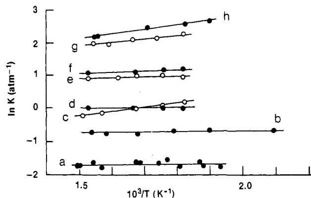
Figure 3. van't Hoff plots for proton-transfer equilibria between the reactants: a. \text{C}_6\text{H}_5\text{CH}_3\text{H}^+ + \text{CH}_2\text{HCOO} ; b. \text{pyridineH}^+ + (\text{CH}_3)_2\text{NH} ; c. \text{C}_6\text{H}_5\text{CH}_3\text{H}^+ + \text{C}_2\text{H}_5\text{CN} ; d. \text{HCOOCH}_3\text{H}^+ + \text{CH}_2\text{CHCN} ; e. \text{CH}_3\text{CNH}^+ + \text{CH}_2\text{CHCN} ; f. \text{CH}_3\text{CNH}^+ + \text{HCOOCH}_3 ; g. \text{pyrroleH}^+ + 2\text{-Fpyridine} ; and h. \text{CH}_3\text{COOCH}_3\text{H}^+ + \text{CH}_3\text{SCH}_3 .
